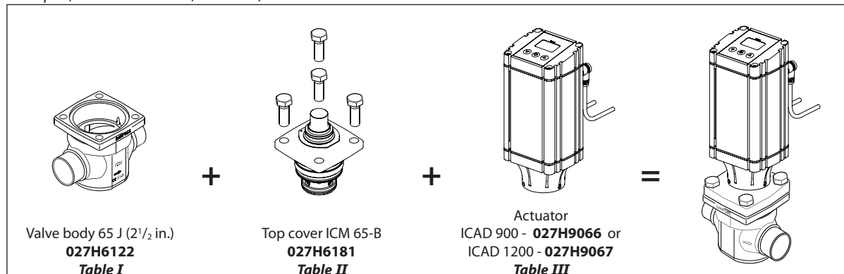
ICV 65 valve body w/different connections
