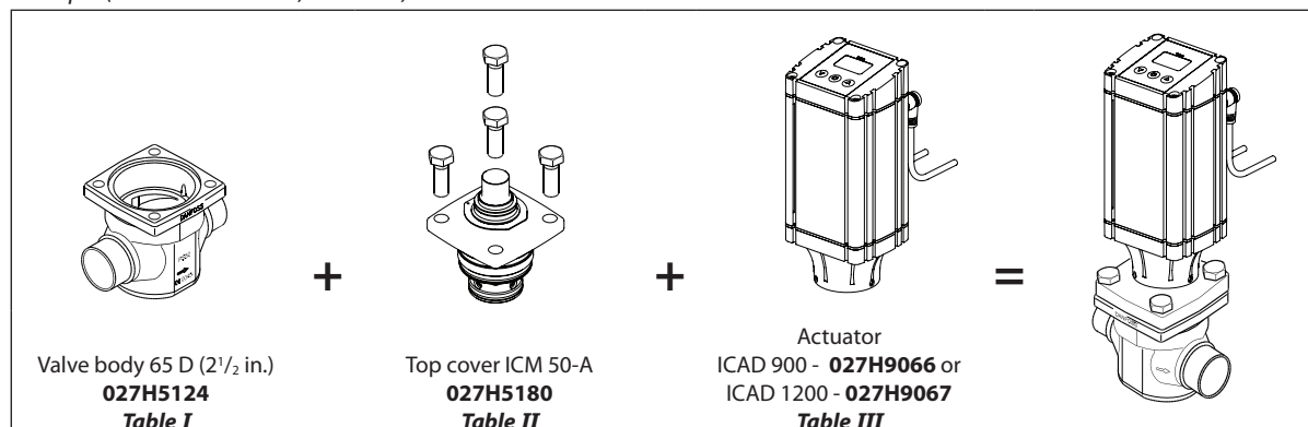
ICV 50 valve body w/different connections
