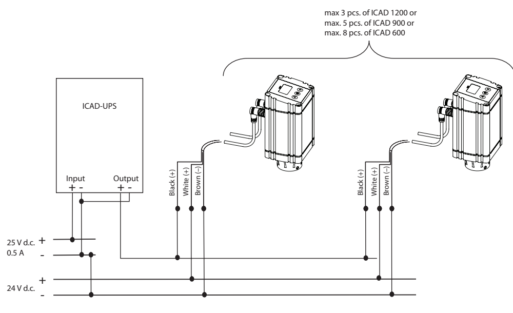
Seperate 24 V d.c tranformer for both ICAD-UPS and ICAD 600/900/1200
