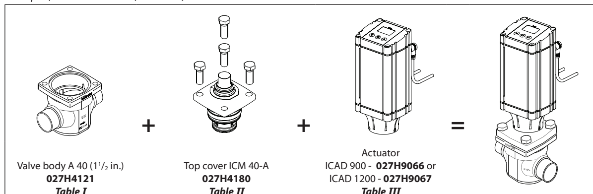
ICV 40 valve body w/different connections
