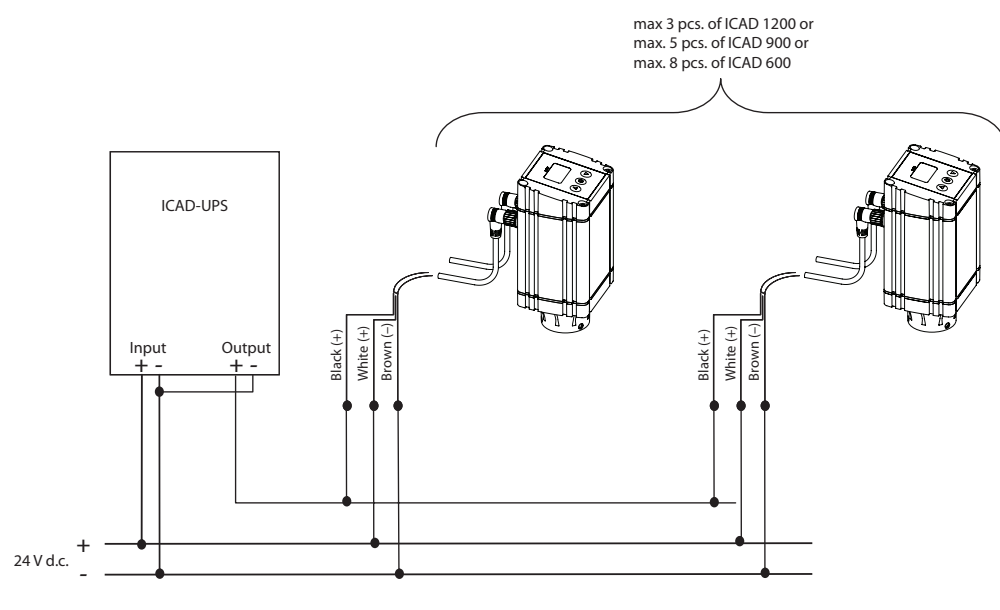
One 24 V d.c tranformer for ICAD-UPS and ICAD 600/900/1200
