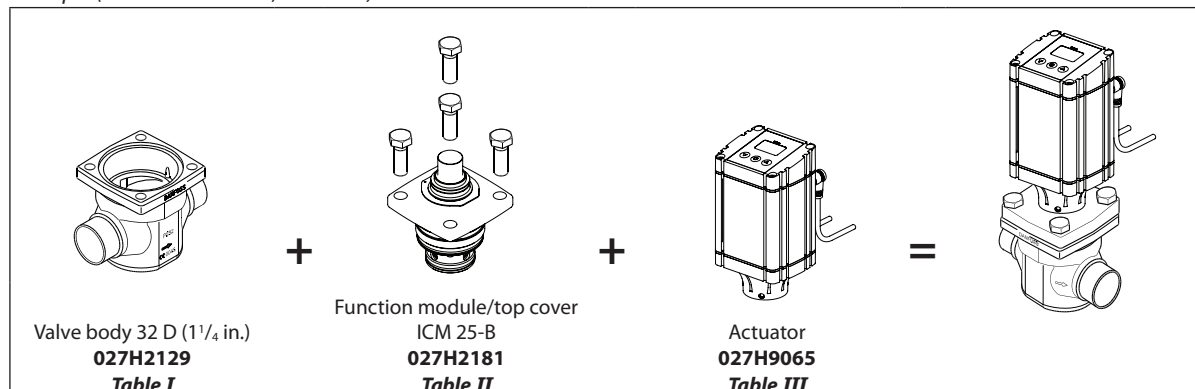
ICV 25 valve body w/different connections
