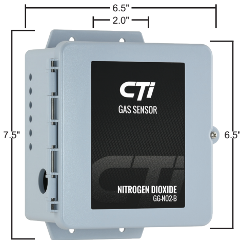
Figure 1: Mounting Dimensions
