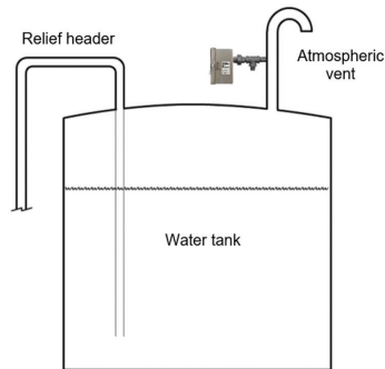
Figure 2: Discharge to Diffusion Tank
