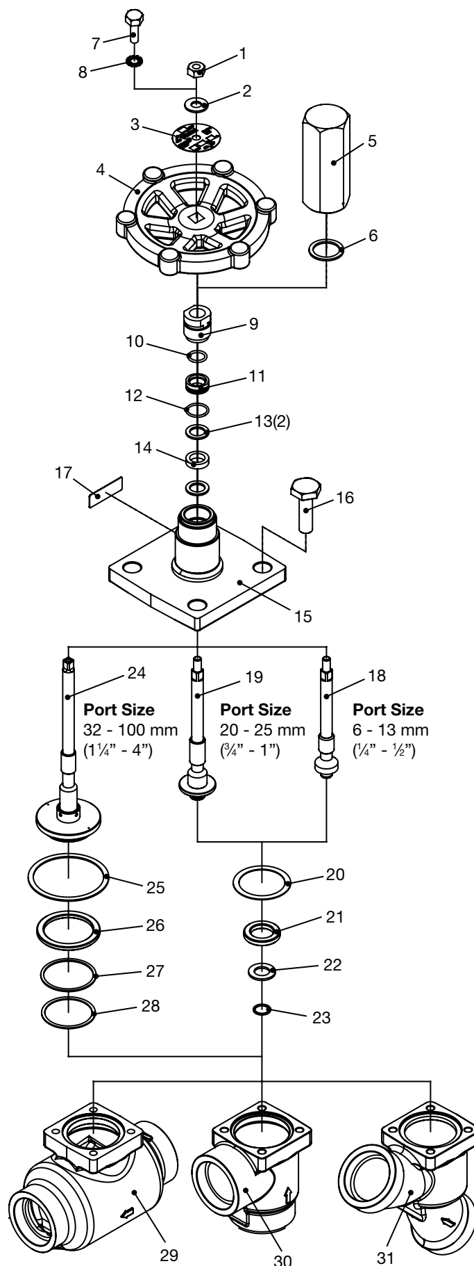
Explosion View: Socket Weld (SW) Standard Bonnet Valves
